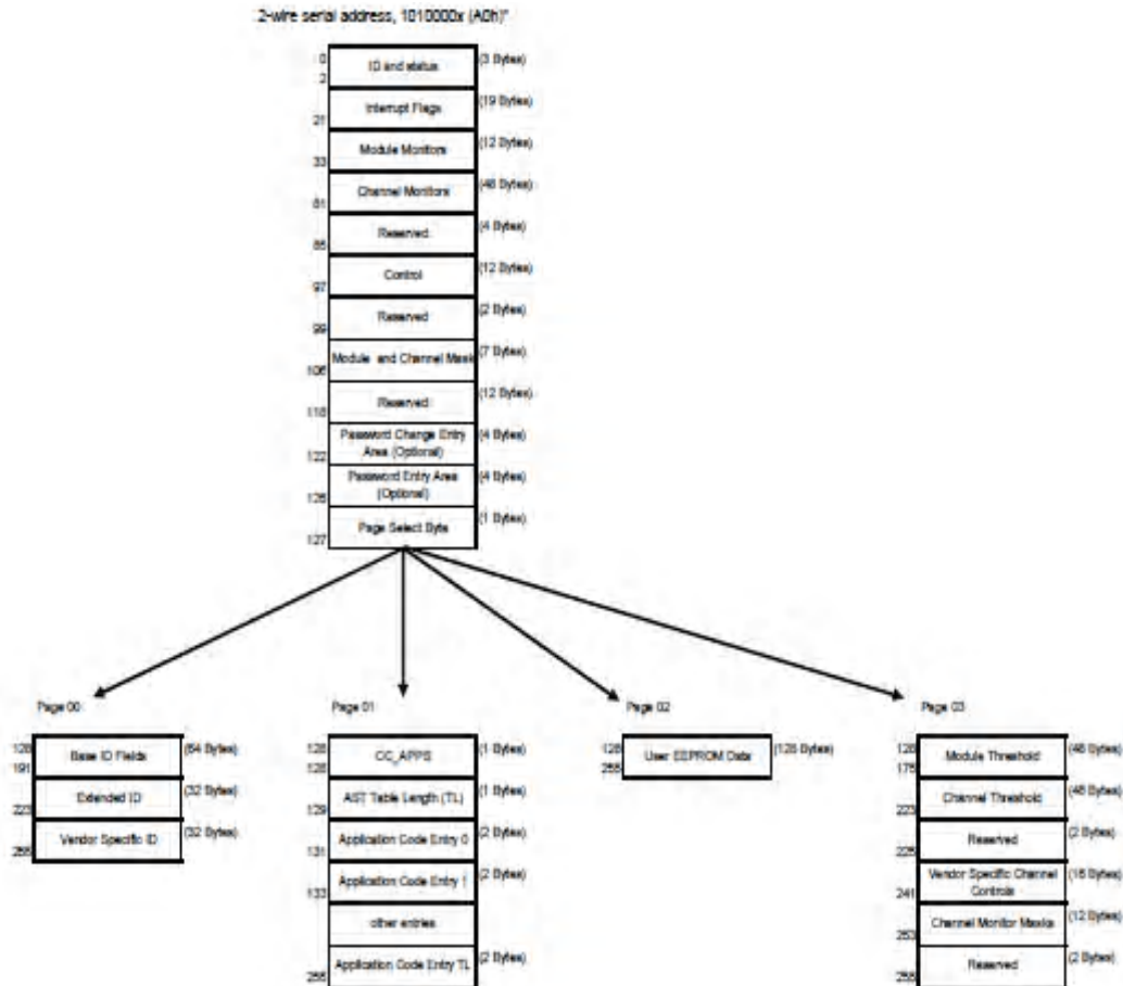
Figure 2 –QSFP+ Memory Map
